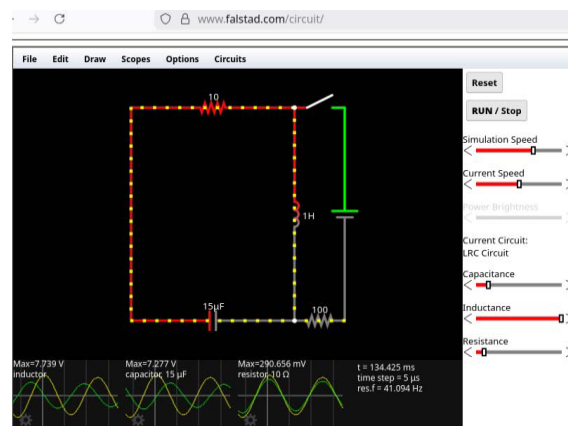
Fig.2 Interfață program simulator circuite electronice.
